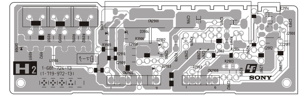
~ H2 Printed Wiring Board Conductor side ~
