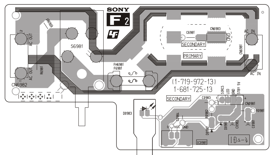
~ F2 Printed Wiring Board Conductor side ~
